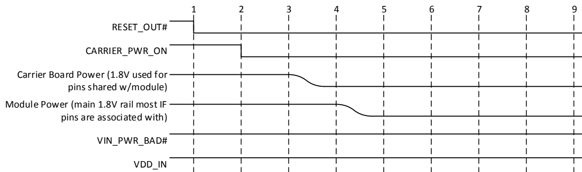
Figure 4 Power Down Sequence
