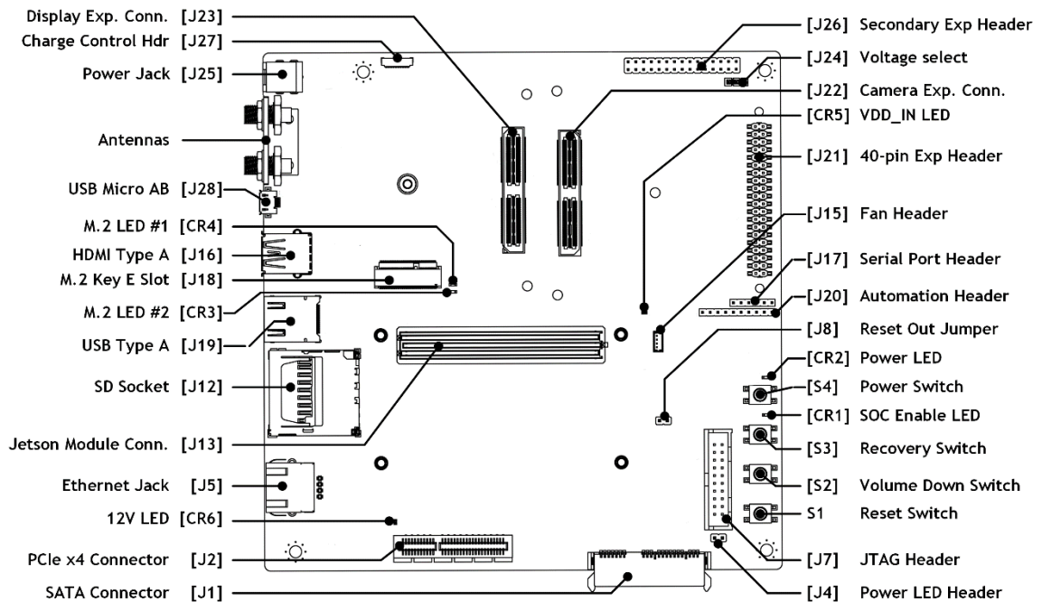
Top view of developer kit carrier board (revision C02)
